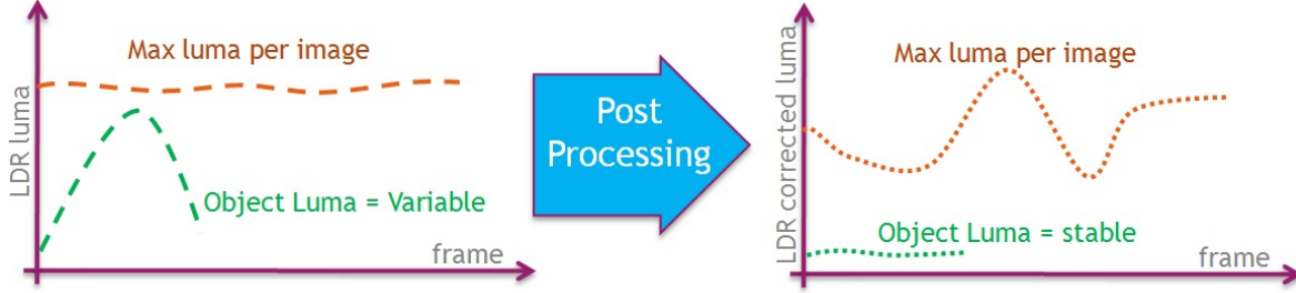
Figure 5: Post processing. The LDR luma is the output of the TMO, see Fig. 3. The object luma (green line) variations have been reduced allowing a perception of the object through time stable. The maximum LDR luma (orange line) is reduce to a smaller range in order to preserve temporal brightness coherency.
